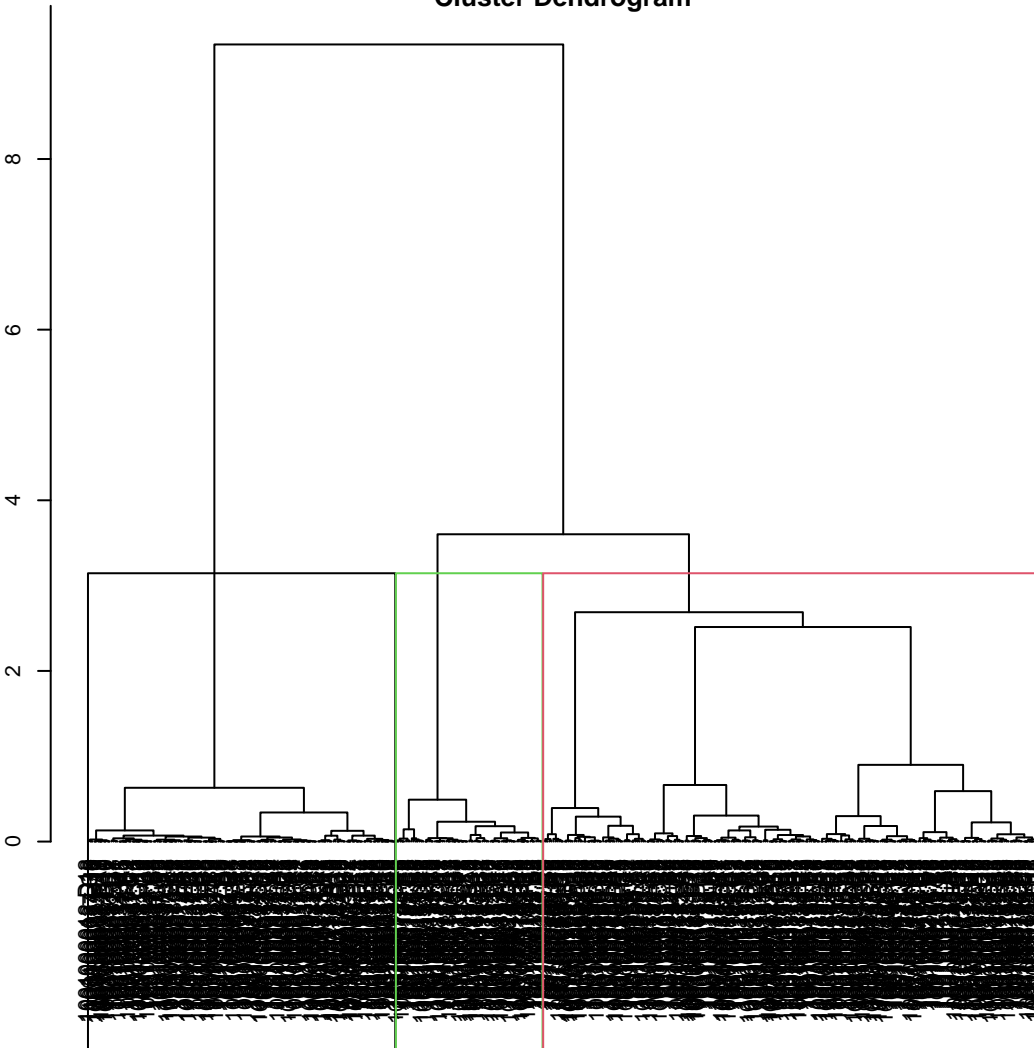
Cluster Dendrogram
