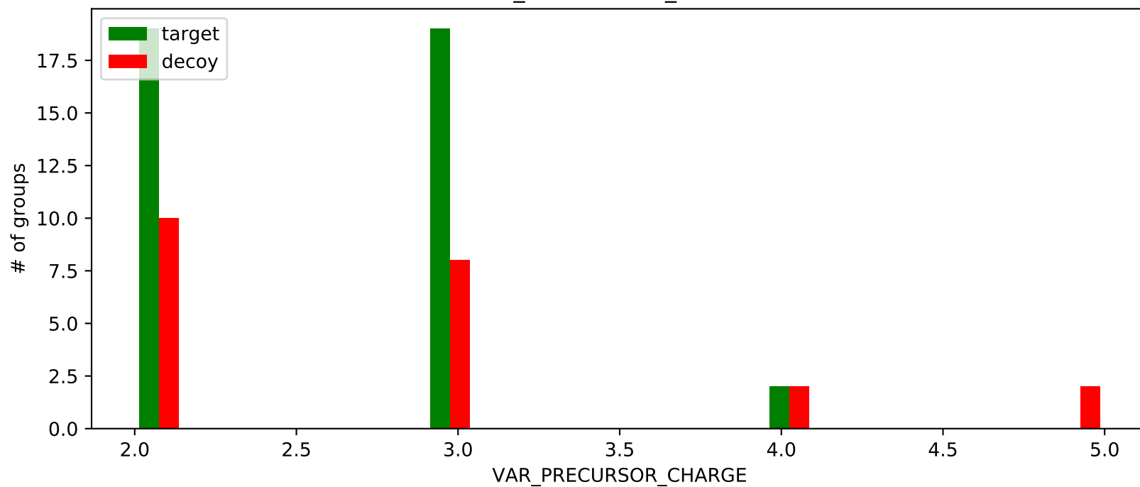
VAR_PRECURSOR_CHARGE
