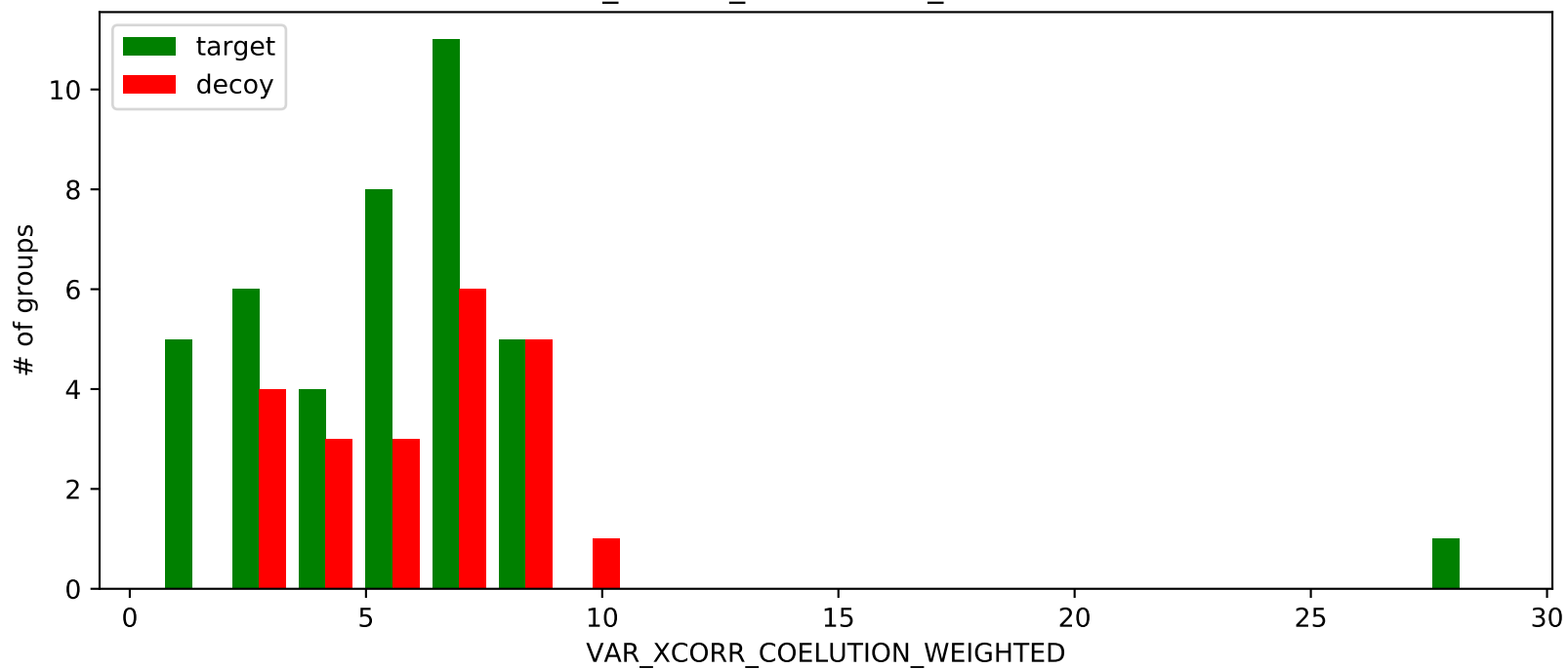
VAR_XCORR_COELUTION_WEIGHTED
