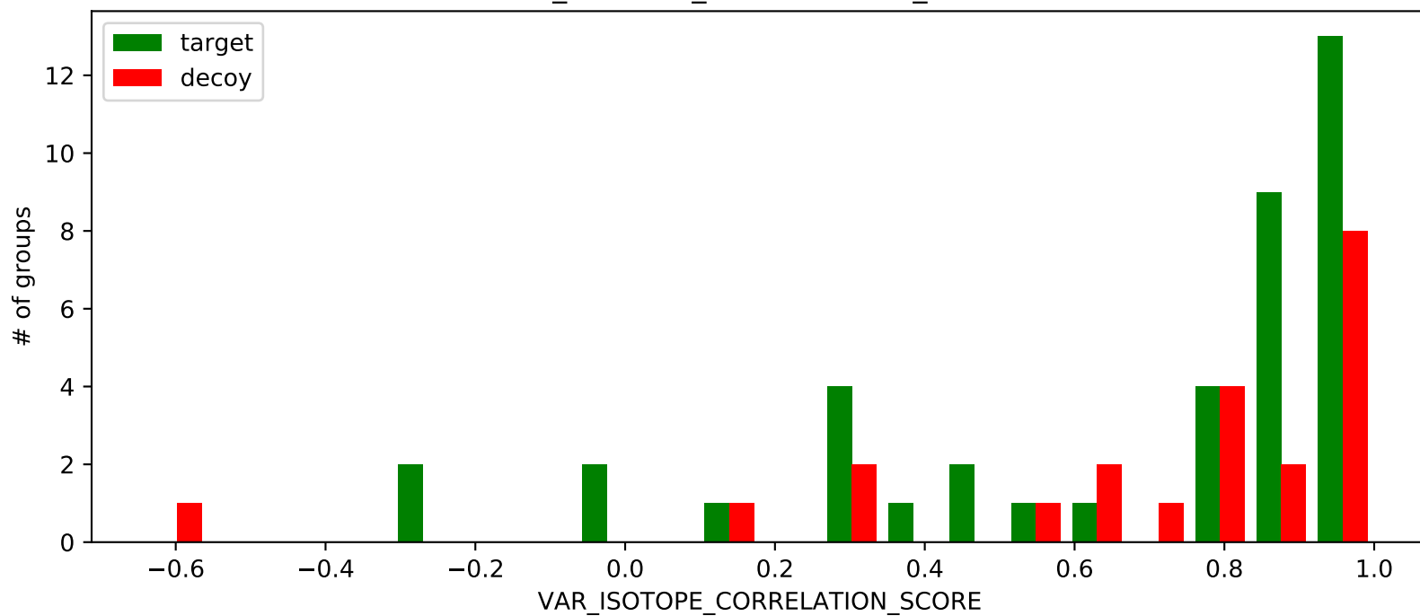
VAR_ISOTOPE_CORRELATION_SCORE
