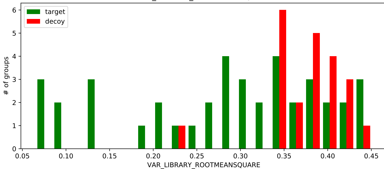
VAR_LIBRARY_ROOTMEANSQUARE
