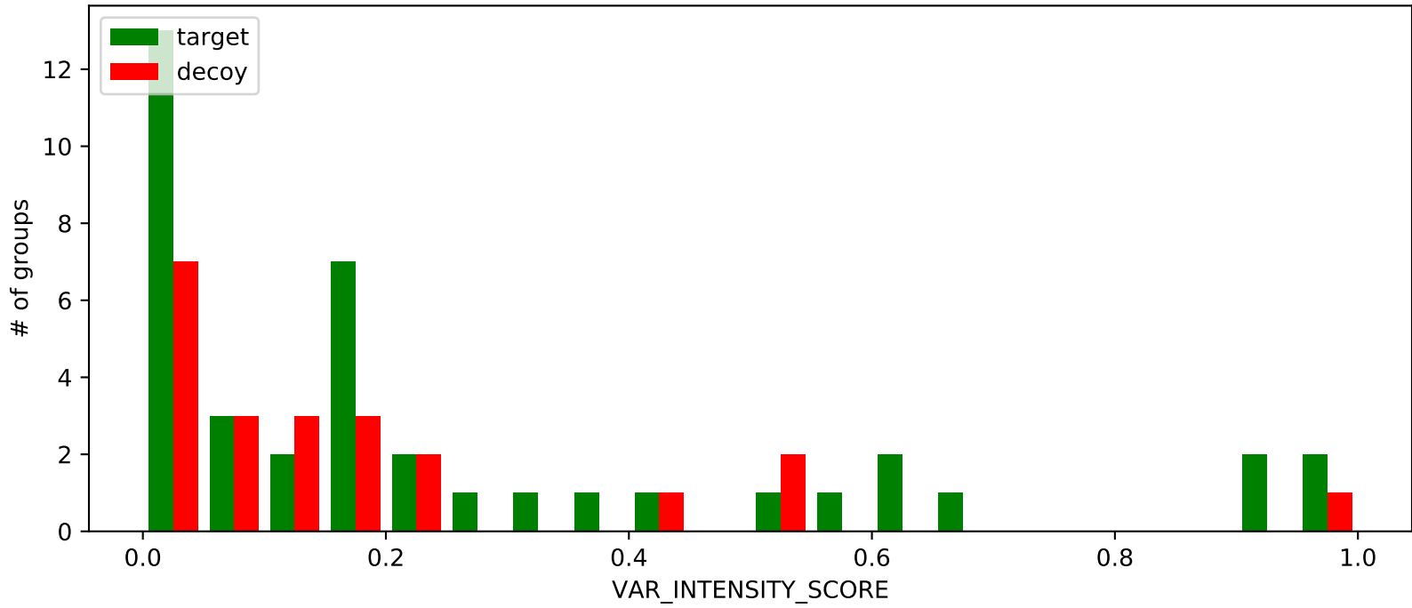
VAR_INTENSITY_SCORE
