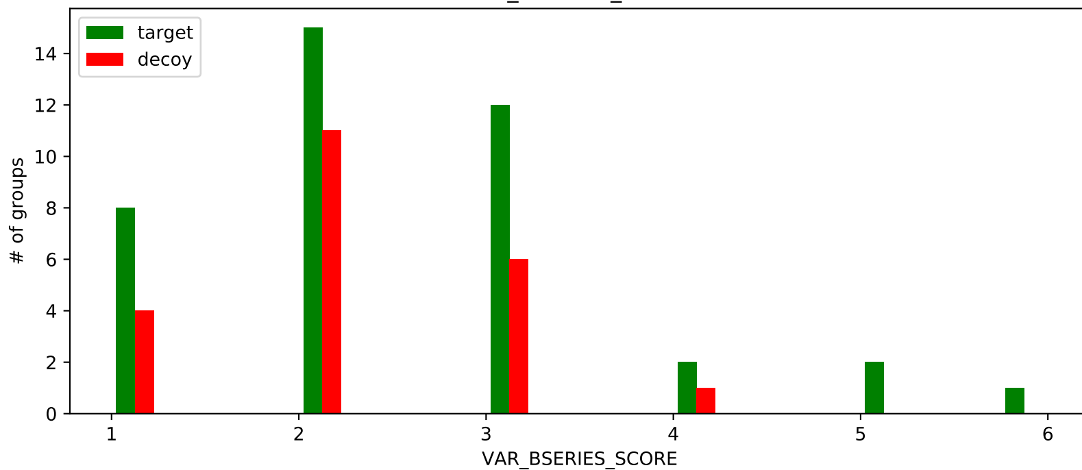
VAR_BSERIES_SCORE
