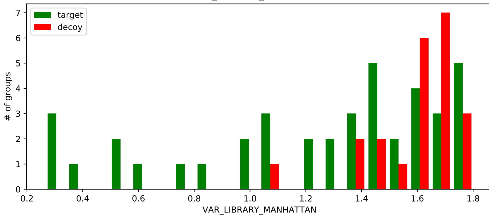
VAR_LIBRARY_MANHATTAN
