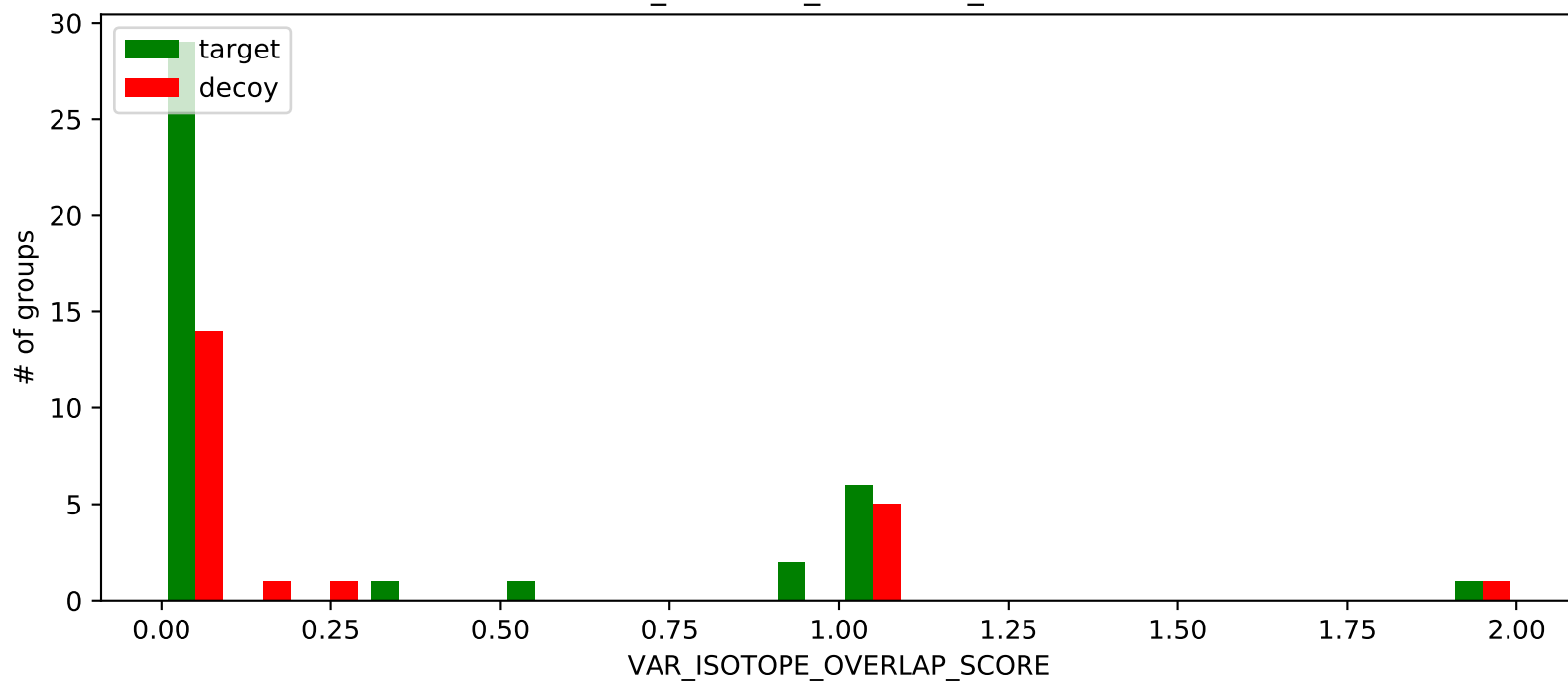
VAR_ISOTOPE_OVERLAP_SCORE
