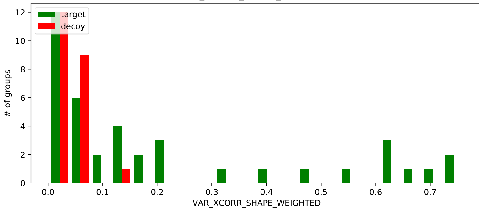
VAR_XCORR_SHAPE_WEIGHTED
