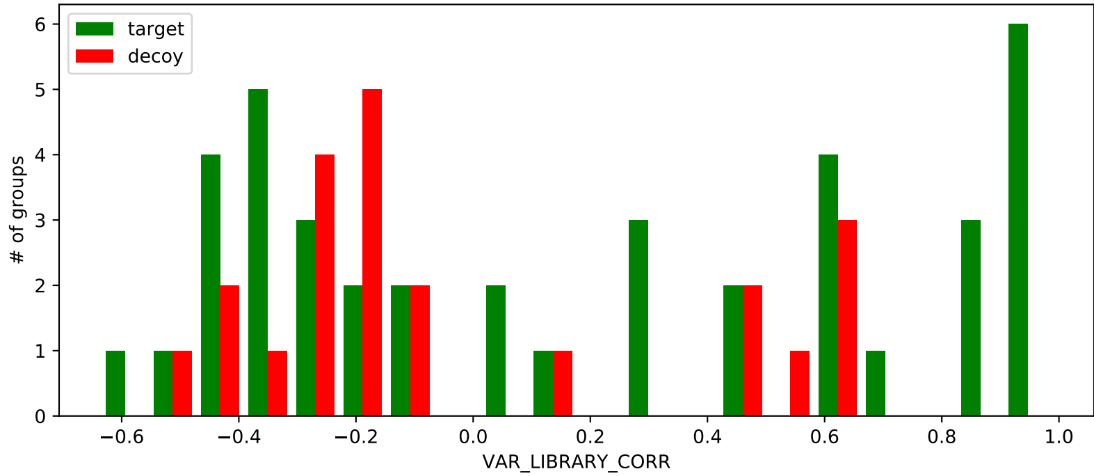
VAR_LIBRARY_CORR
