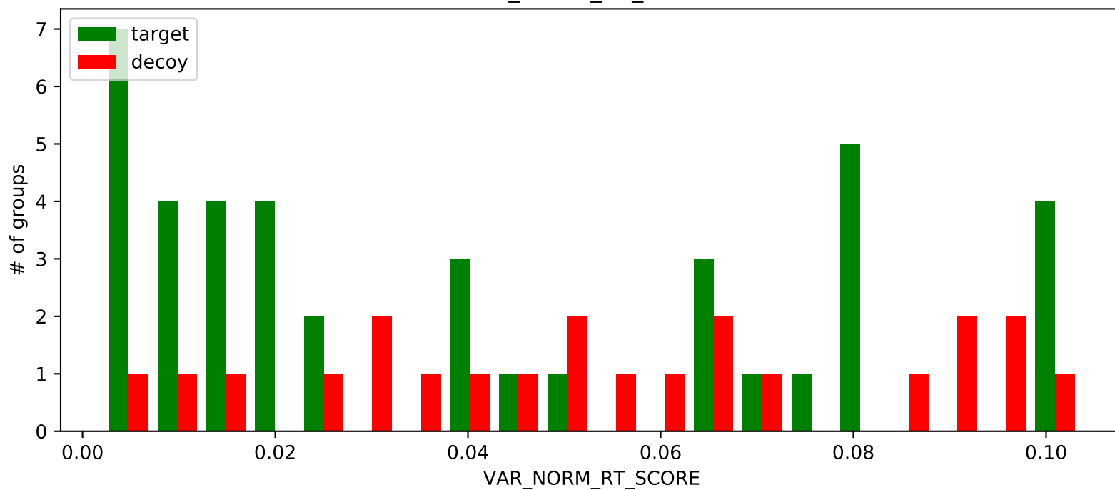
VAR_NORM_RT_SCORE
