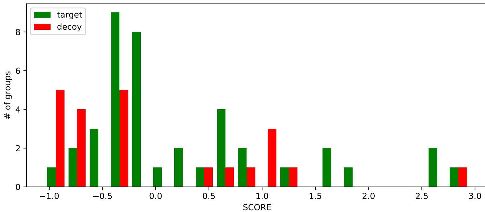
SCORE
