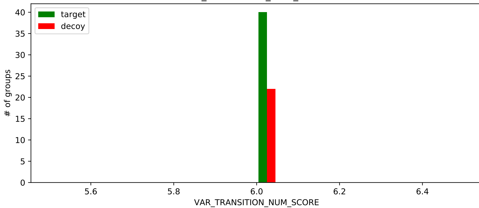
VAR_TRANSITION_NUM_SCORE
