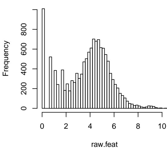
ExpData Log(NumFeat)
