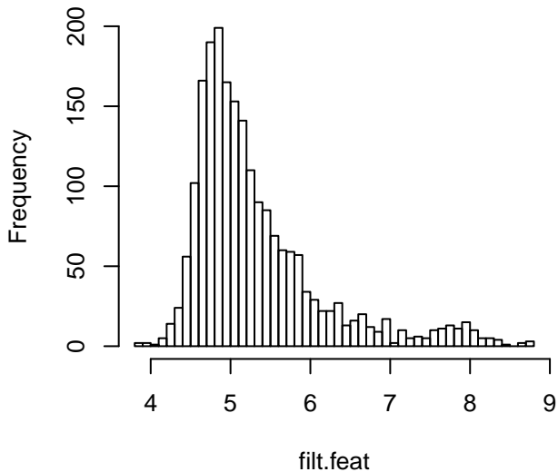
FiltData Log(NumFeat)
