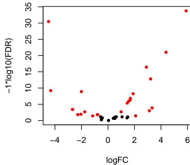
Volcano plot
