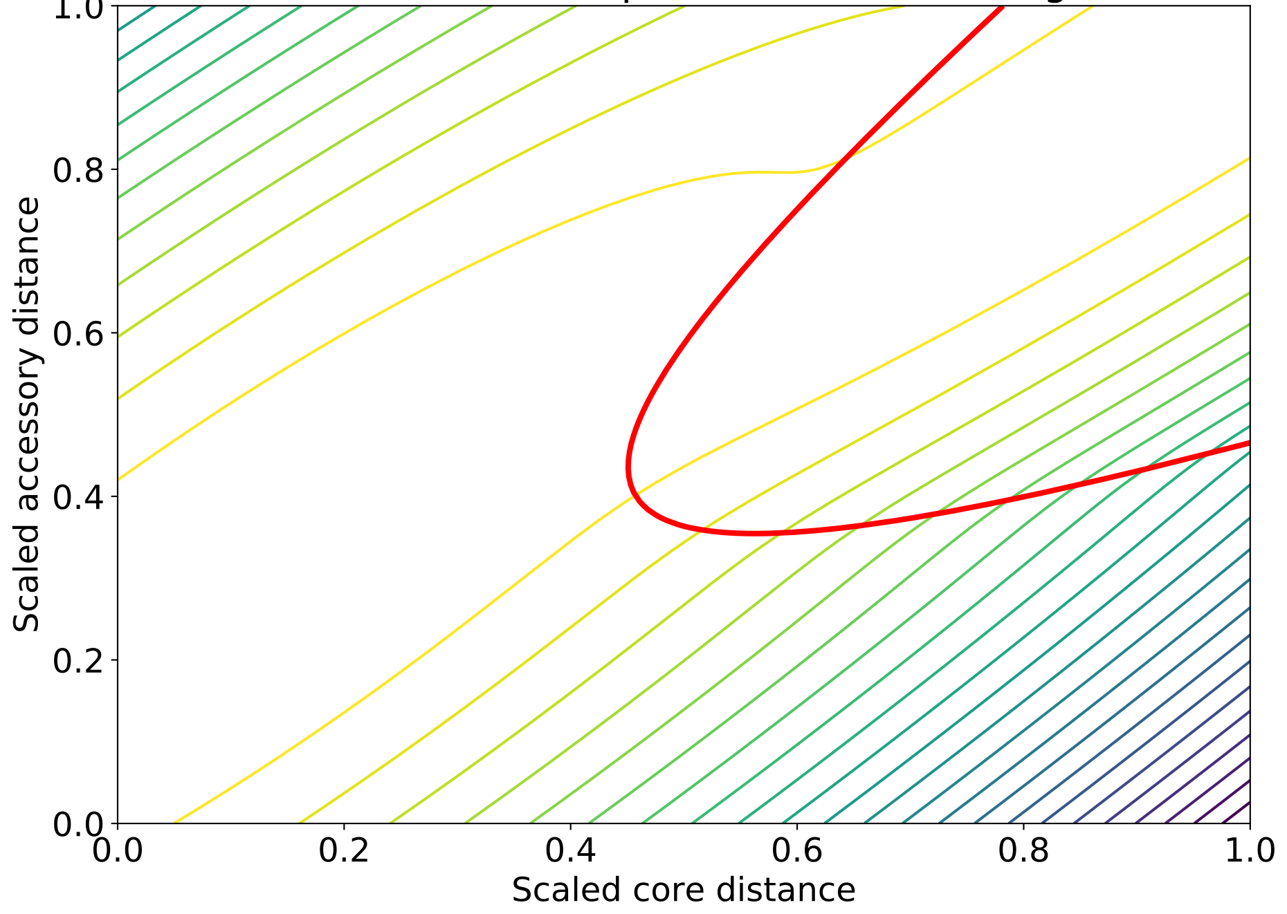
DPGMM - estimated number of spatial clusters: 2 assignment boundary
