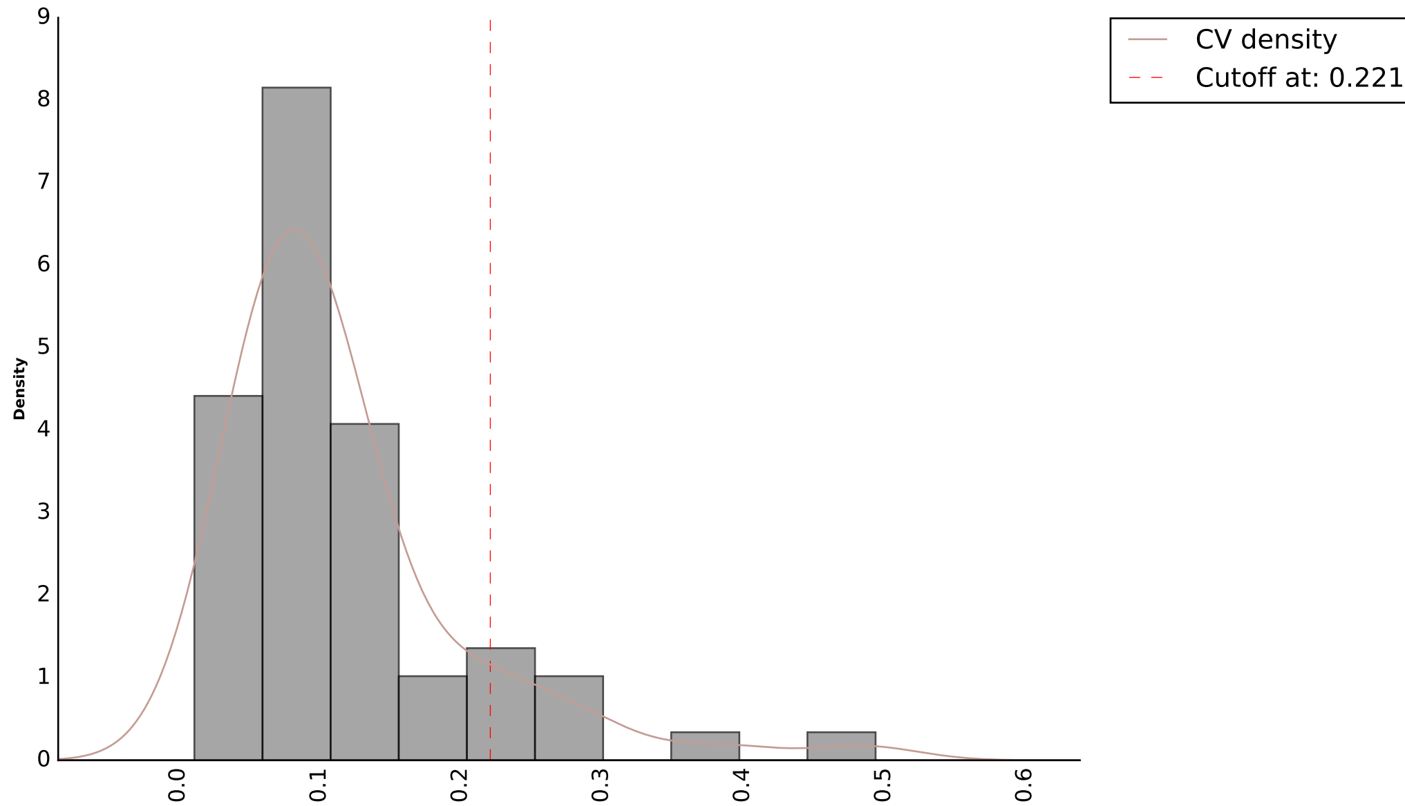
Density Plot of Coefficients of Variation in Pinot gris, Napa, CA 2004
