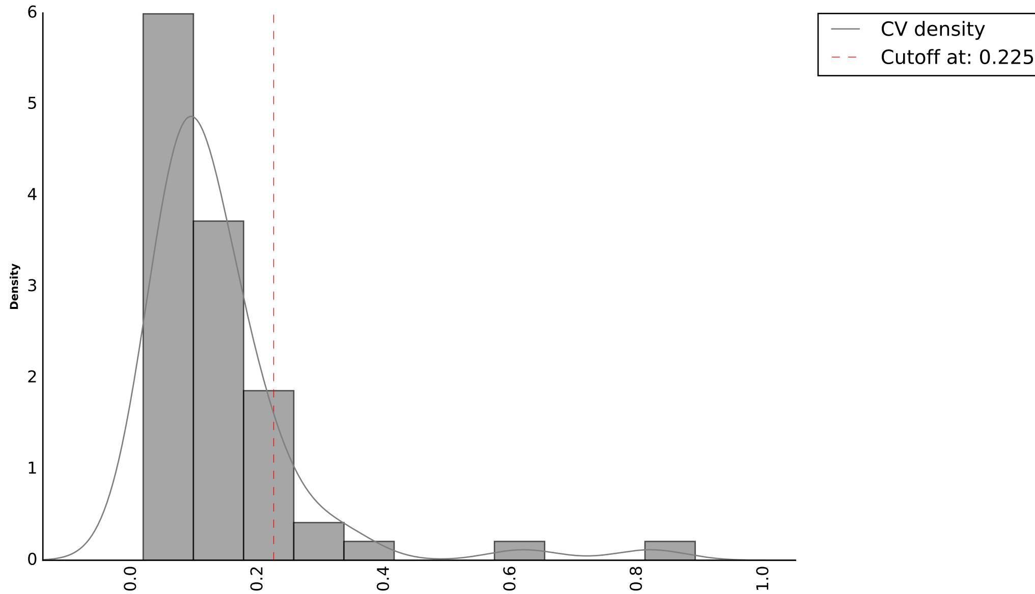
Density Plot of Coefficients of Variation in Fume Blanc, Napa, CA 2004
