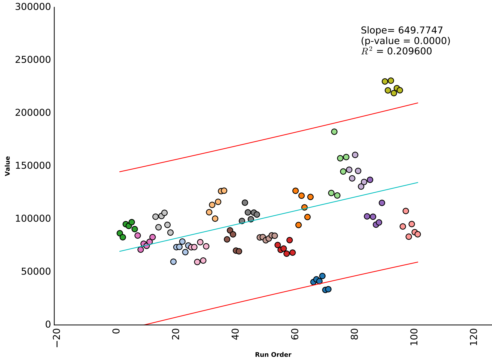
_667682 Scatter plot (fitted regression line and prediction bands included)
