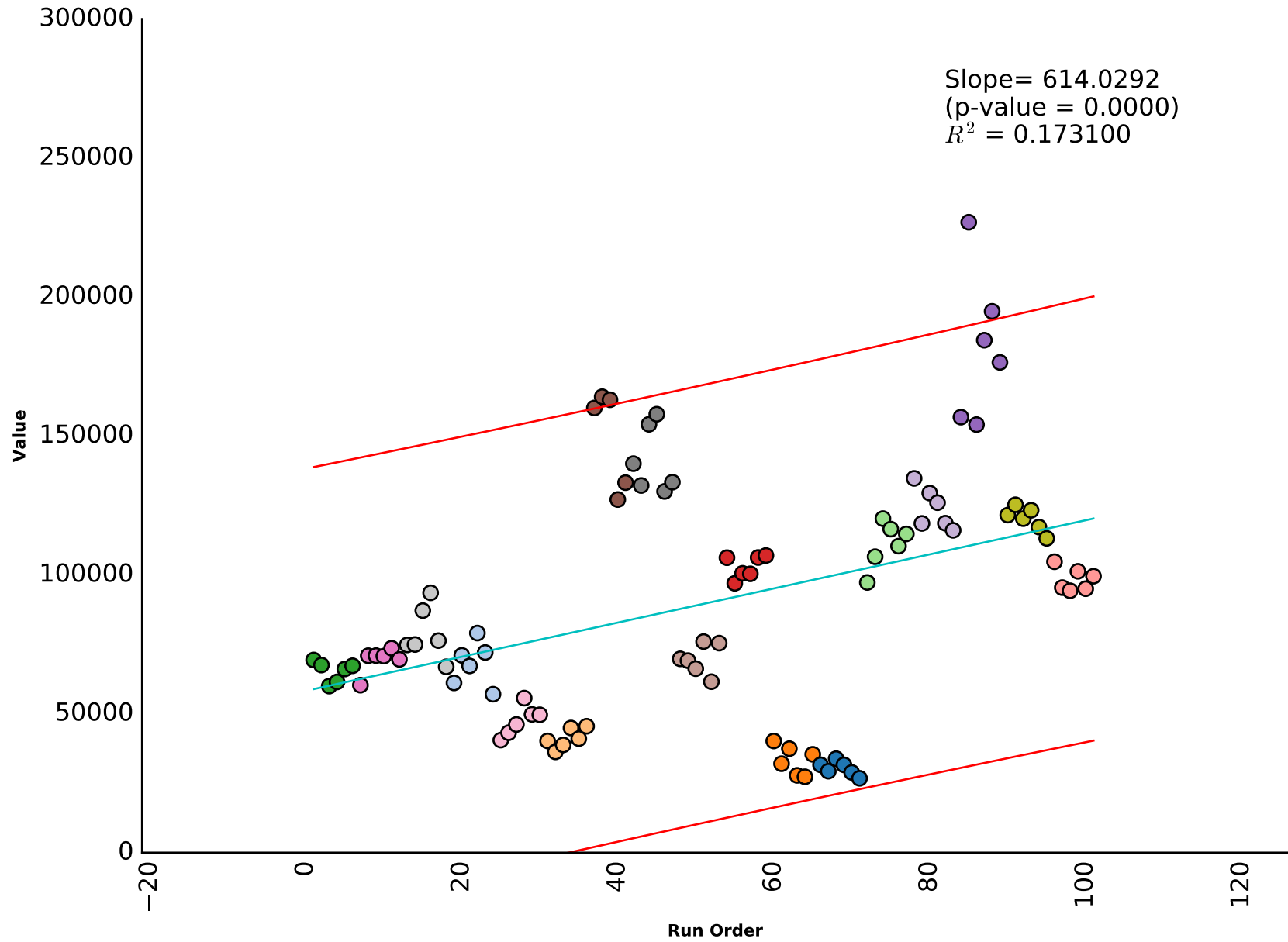
_506359 Scatter plot (fitted regression line and prediction bands included)
