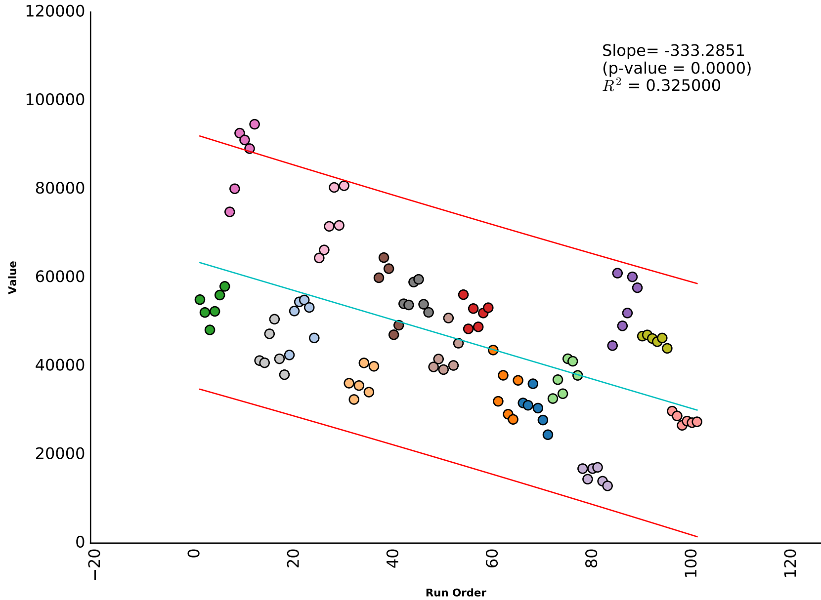
_663088 Scatter plot (fitted regression line and prediction bands included)
