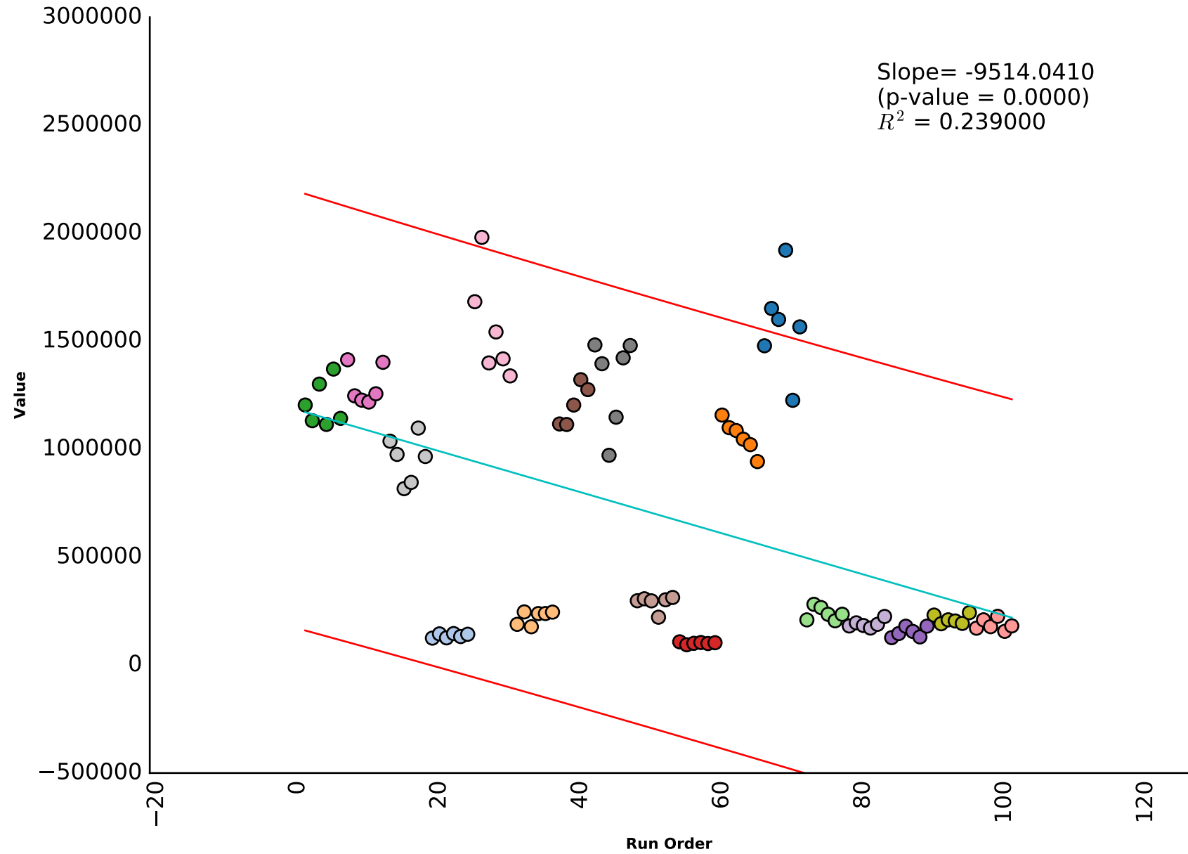
_216442 Scatter plot (fitted regression line and prediction bands included)
