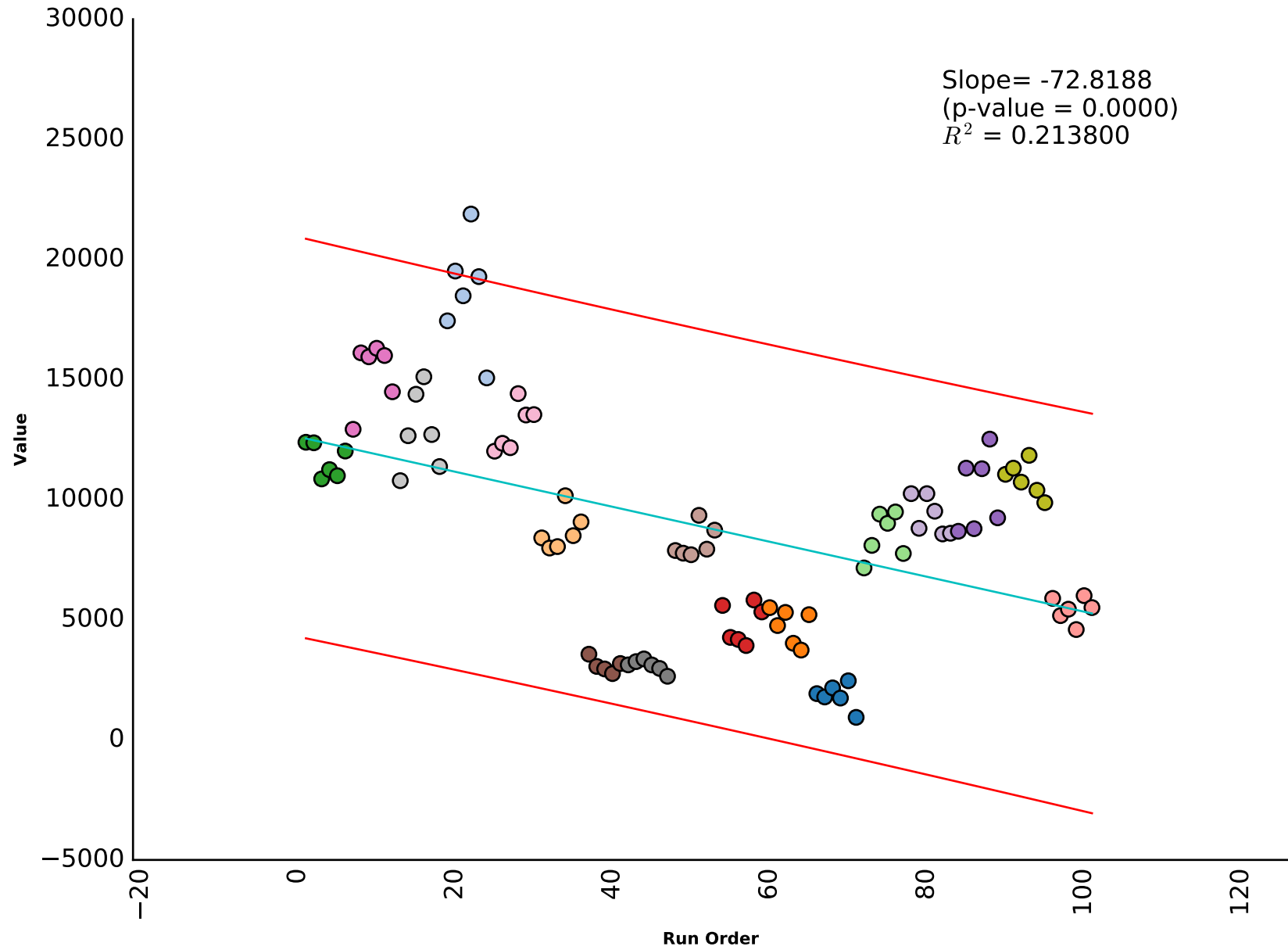
_435138 Scatter plot (fitted regression line and prediction bands included)
