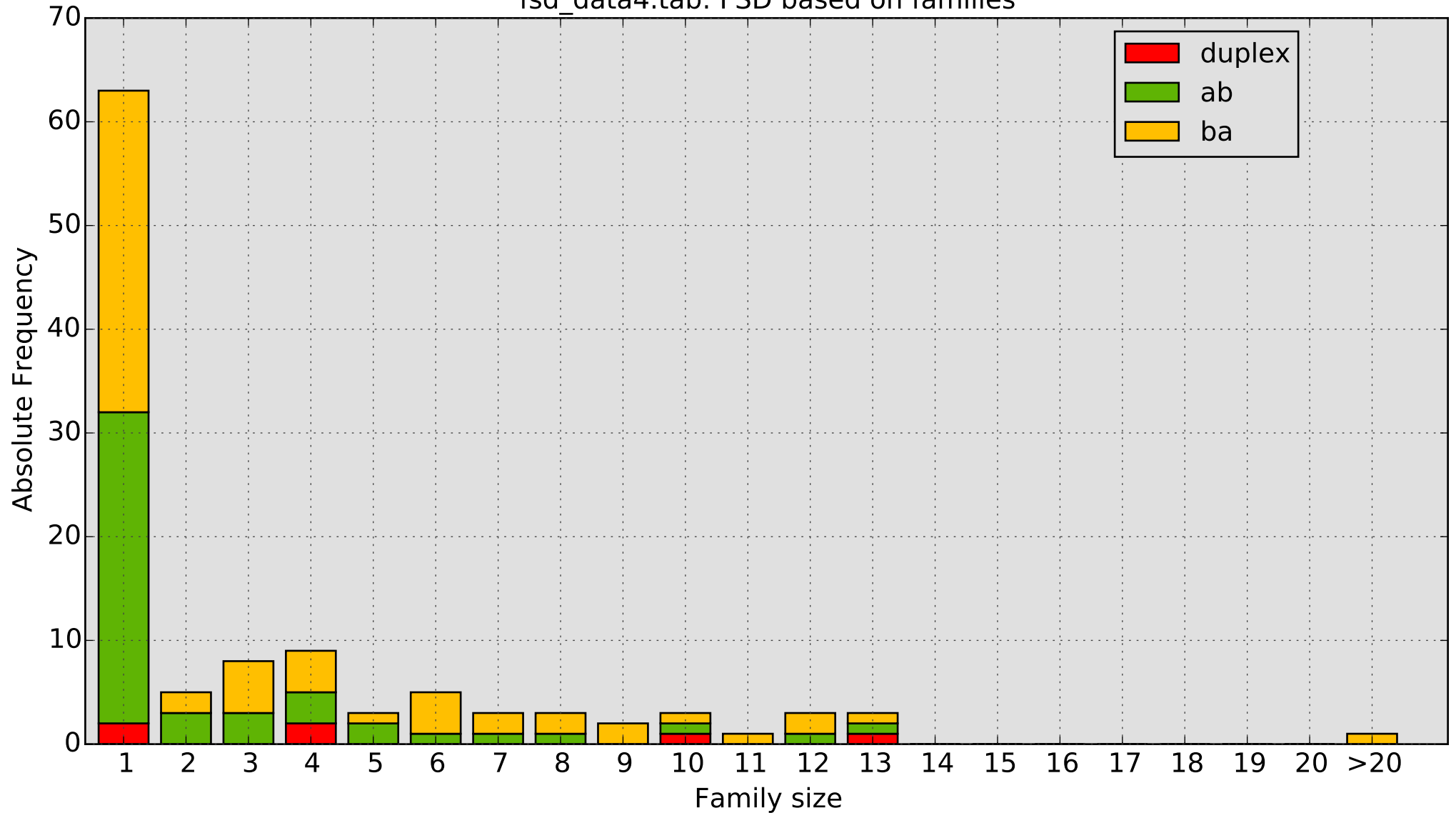
fsd_data4.tab: FSD based on families
