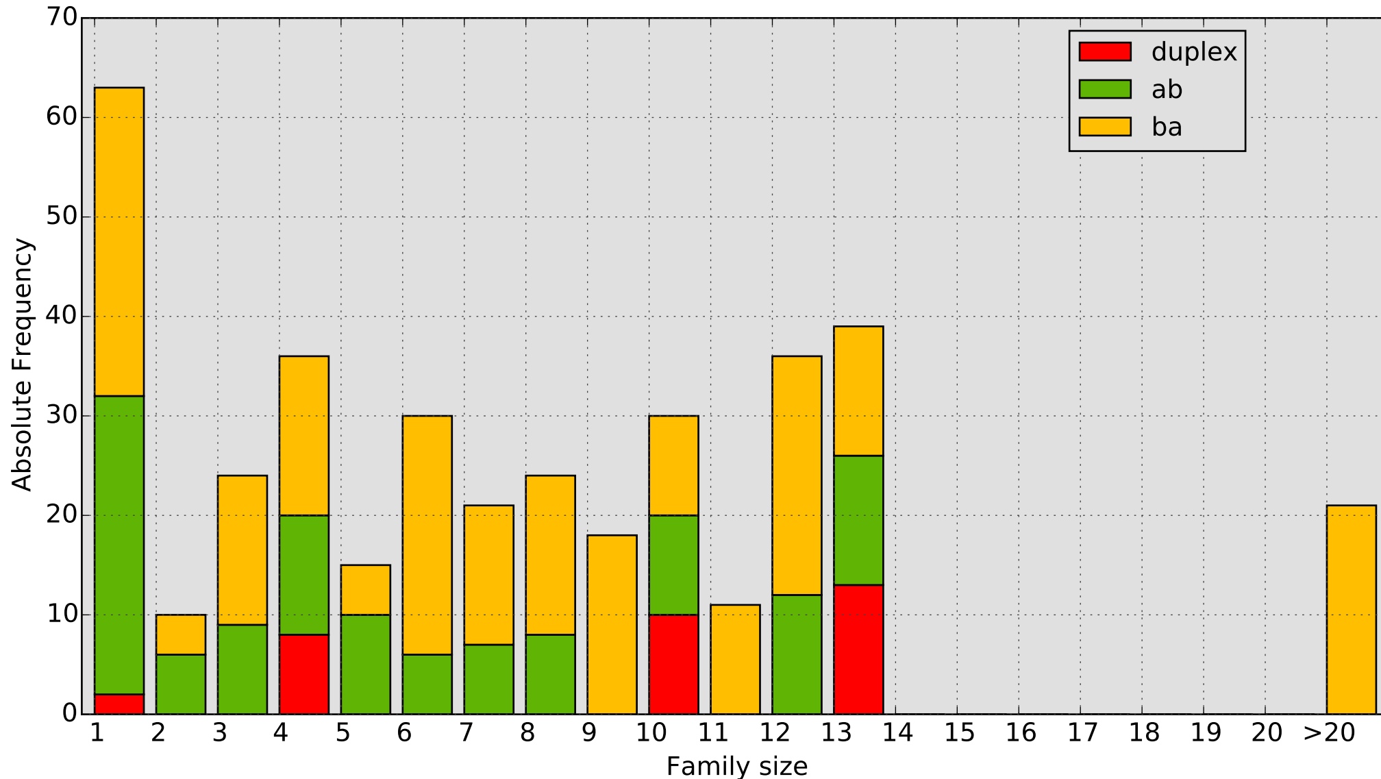
fsd_data4.tab: FSD based on PE reads
